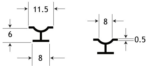
Sliding Door Ultra Lower Track (7H x 12W)
