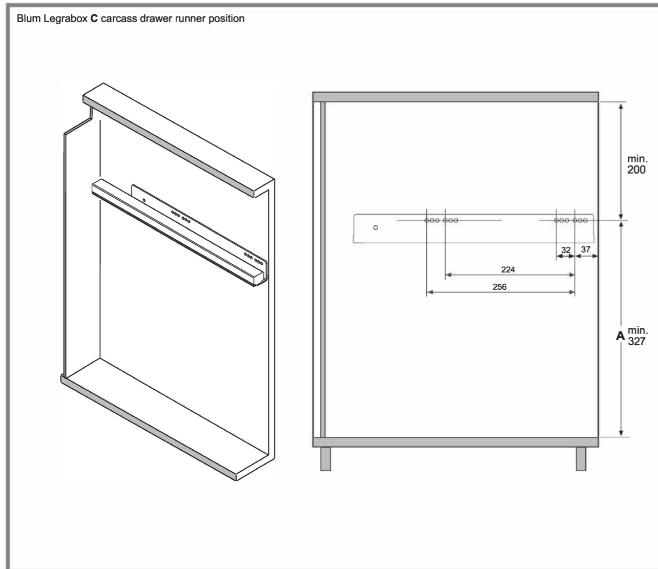
Blum Legrabox C drawer front drilling position
