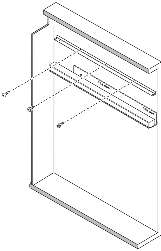
Blum Legradox C carcass drawer runner & metal lid position
