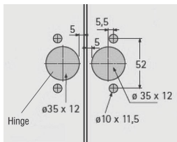
Extra centre hinge dimensions
